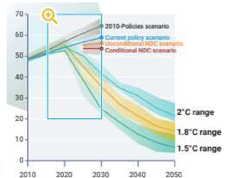
Figure ES.5. Global GHG emissions under different scenarios and the emissions gap in 2030 (median and 10 th to 90 th percentile range; based on the pre-COVID-19 current policies scenario)
